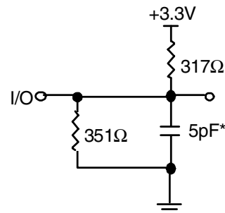
Figure 2. High-Impedance Test Load (for t_{OH} , t_{CH} , t_{OL} , and t_{DC1} )
